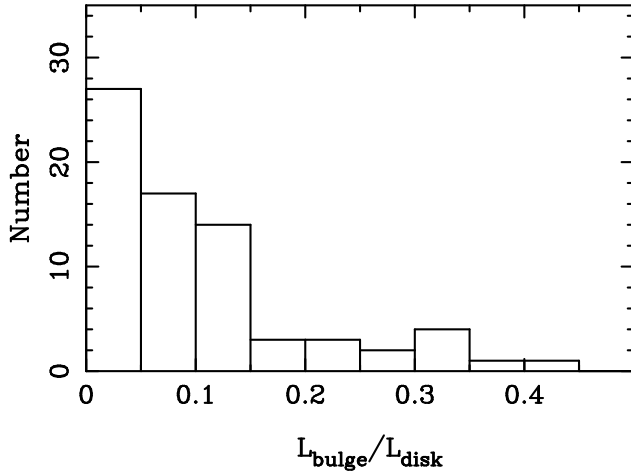
Fig. 5. Bulge to the disk luminosity ratio. Most late-type spiral galaxies do not have a very bright bulge. (Data from Palunas, Williams 2000).
